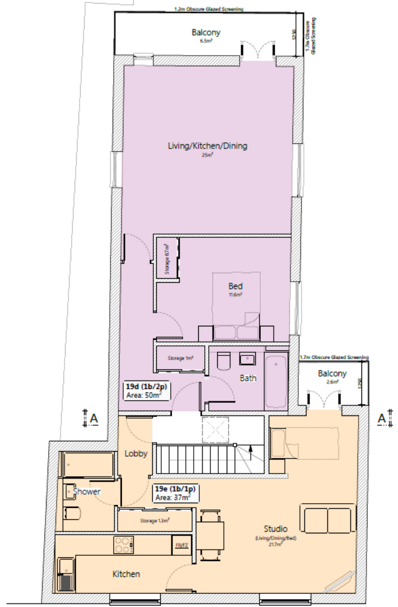
Second Floor Scale: 1:50 @ A2
