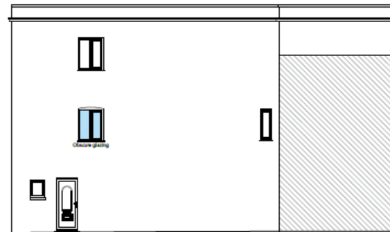
South West Elevation Scale: 1:100 @ A2
