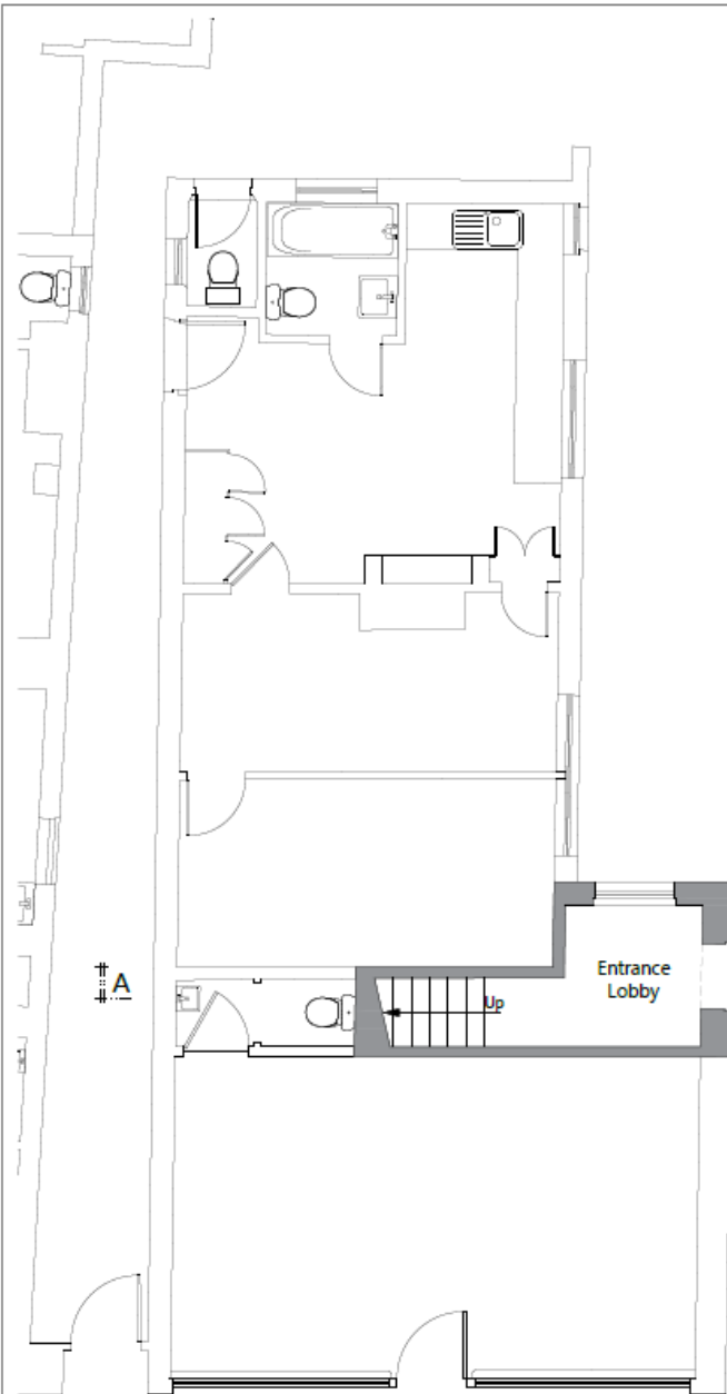
Ground Floor Scale: 1:50 @ A2
